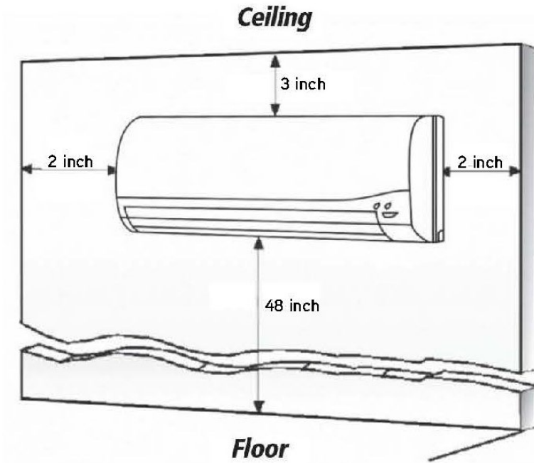
Fig 1: Minimum clearances for the high-wall indoor unit
