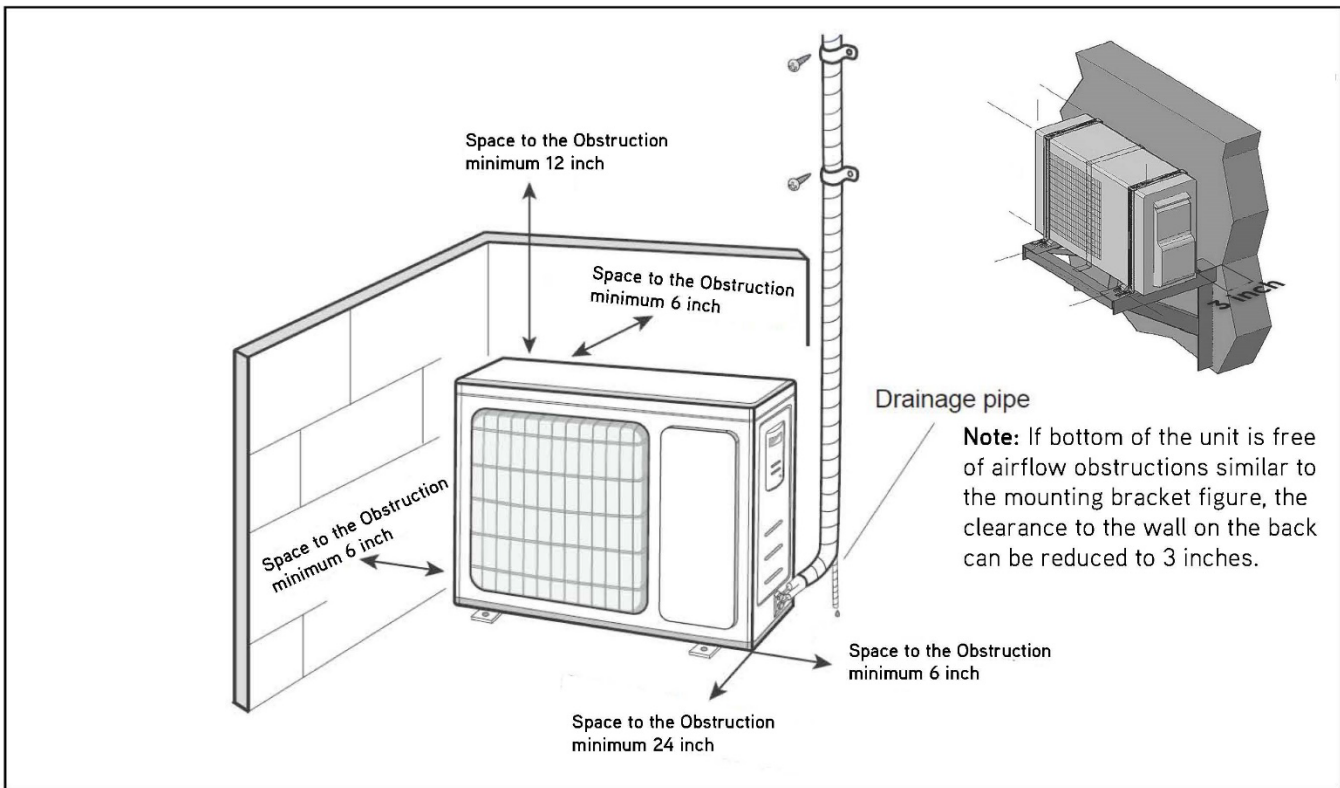
Fig 2: Minimum clearances for the outdoor unit
