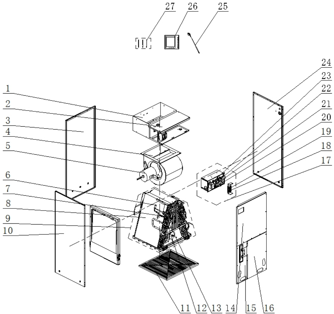
Exploded View of GMV-ND48A/B-T(U) / GMV-ND54A/B-T(U) / GMV-ND60A/B-T(U):
