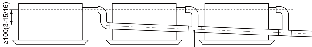
Drainage pipes assembled by T-shaped joints
