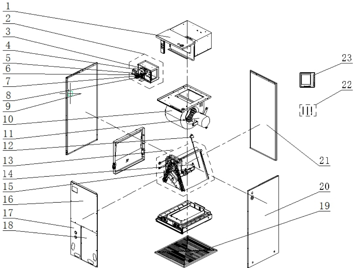
Exploded View of GMV-ND09A/B-T(U) / GMV-ND12A/B-T(U) /GMV-ND18A/B-T(U)/ GMV-ND24A/B-T(U) / GMV-ND30A/B-T(U):
