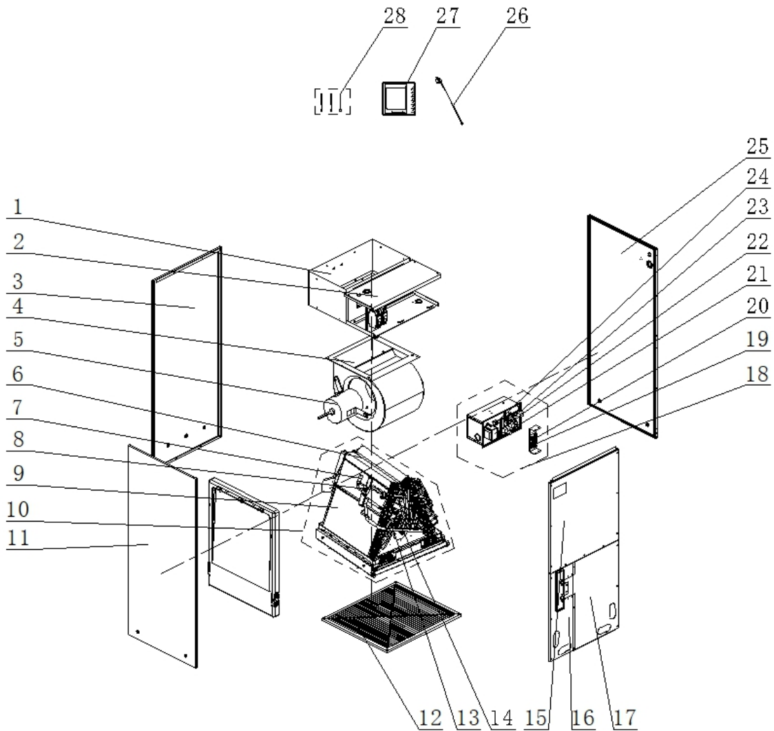
Exploded View of GMV-ND36A/B-T(U) / GMV-ND42A/B-T(U):
