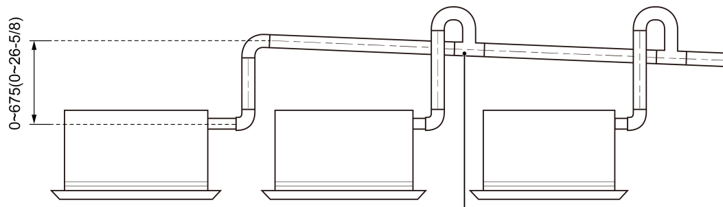
Drainage pipes assembled by T-shaped joints
