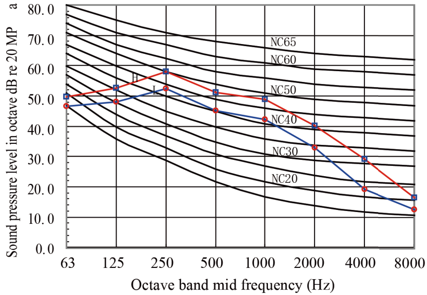
Noise evaluation curve
